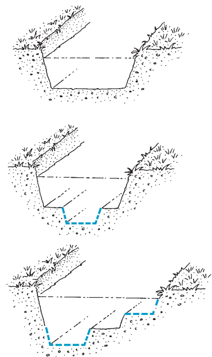
Examples of profiles that can be considered for the new or re-profiled channel.
